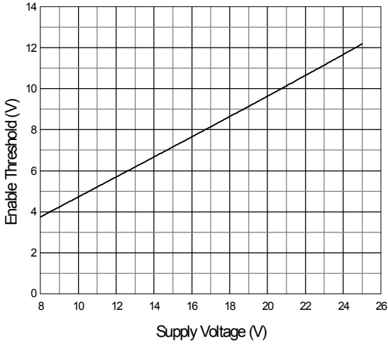
Fig. 21 Enable Threshold vs. Supply Voltage
