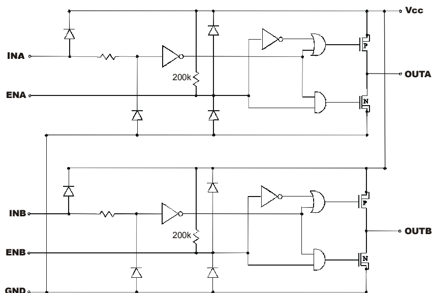
Figure 1 - Functional Diagram
