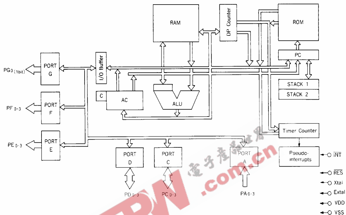
LM6413/6416 Block Diagram
