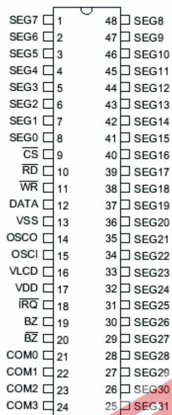
SS1621B-48SSOP
