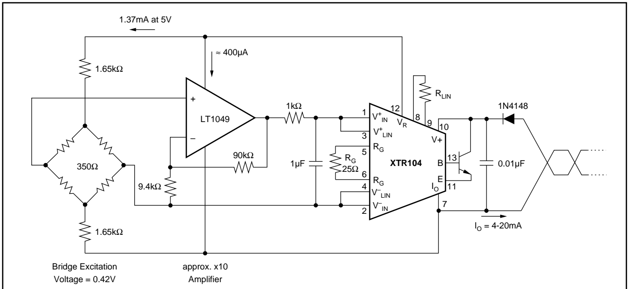
FIGURE 8. 350 \Omega Bridge With X10 Preamplifier.
