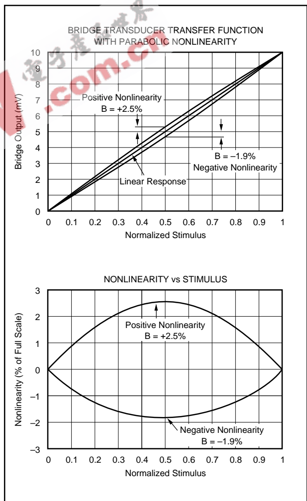
FIGURE 4. Parabolic Nonlinearity.
