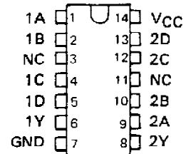
SN5420 . . . J PACKAGE SN54LS20, SN54S20 . . . J OR W PACKAGE SN7420 . . . N PACKAGE SN74LS20, SN74S20 . . . D OR N PACKAGE (TOP VIEW)
