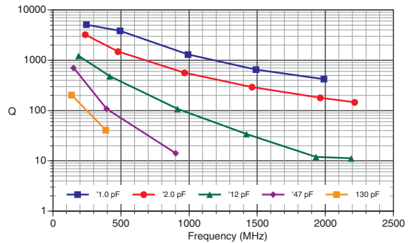
Q Factor: 1210/S41C
