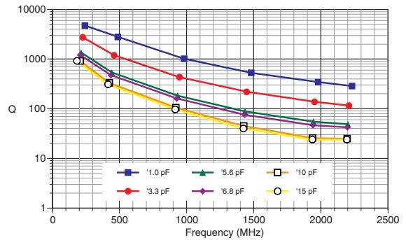
Q Factor: 0603/R14C
