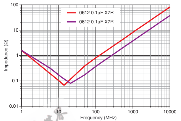
IMPEDANCE 0612 vs. 1206
