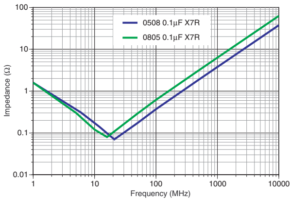
IMPEDANCE 0508 vs. 0805
