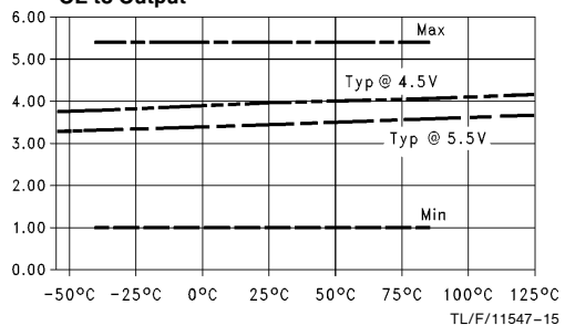
t_{PHZ} vs Temperature ( T_A ) C_L = 50\text{ pF} , 1 Output Switching \text{OE} to Output
