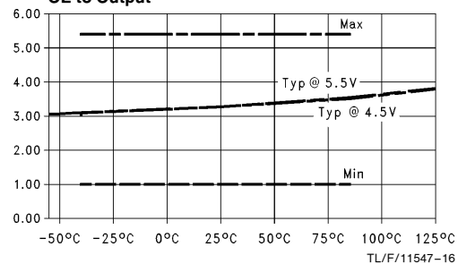
t_{PLZ} vs Temperature ( T_A ) C_L = 50\text{ pF} , 1 Output Switching \text{OE} to Output
