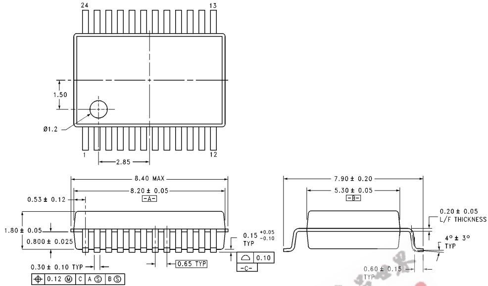
24-Lead Molded Shrink Small Outline, EIAJ, Type II (MSA) NS Package Number MSA24
