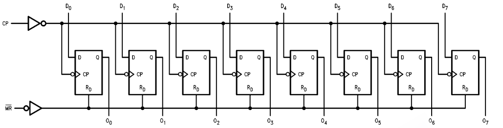
Logic Diagram
