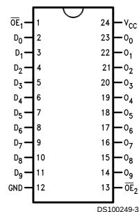
Pin Assignment for DIP and Flatpak
