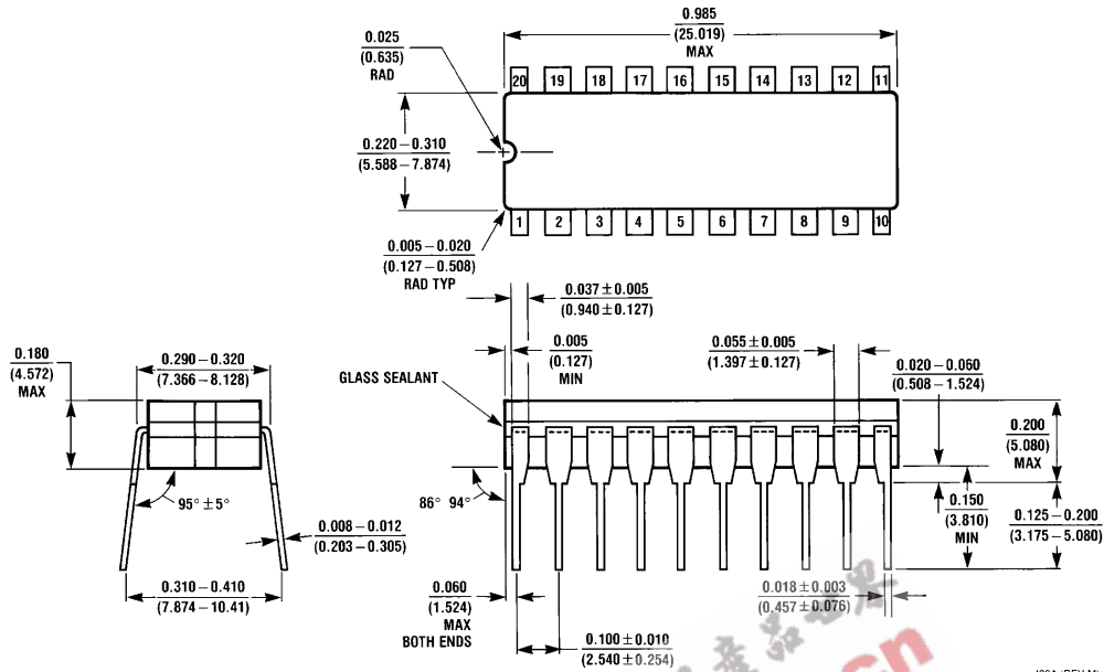
20-Lead Ceramic Dual-In-Line Package (DIP) NS Package Number J20A
