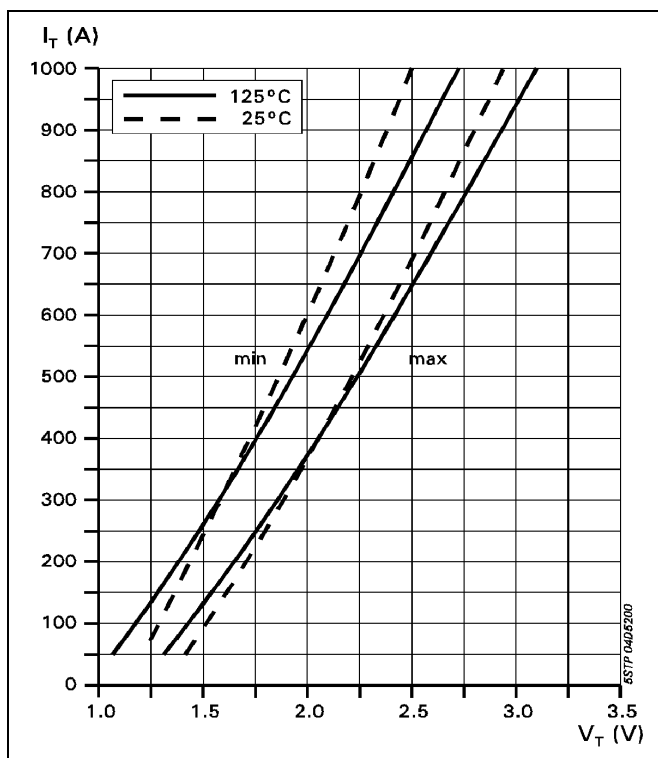
Fig. 2 On-state characteristics.
