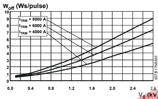
Fig. 17 W_{off} = f(V_0, I_T) , T_j = 125^\circ\text{C} . Half sinusoidal waves. t_p = 10\text{ ms} .
