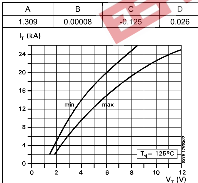
Fig. 2 On-state characteristics.
