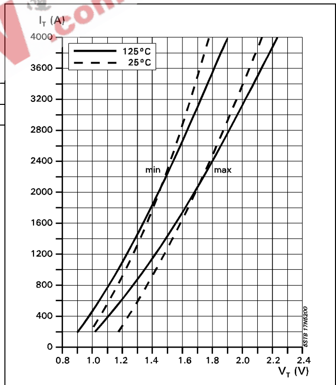
Fig. 3 On-state characteristics.
