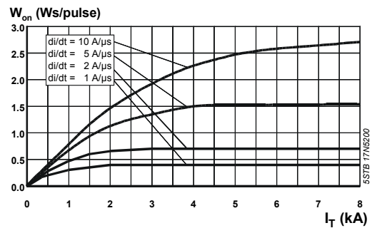
Fig. 16 W_{on} = f(I_T, di/dt) , T_j = 125^\circ\text{C} . Rectangular waves.
