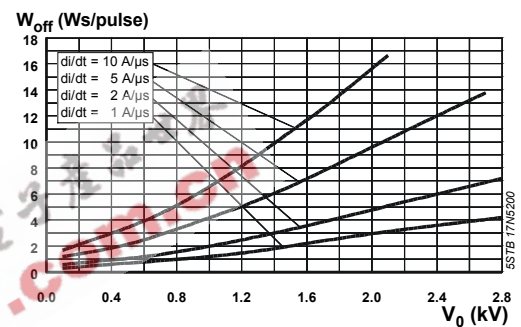
Fig. 18 W_{off} = f(V_0, di/dt) , T_j = 125^\circ\text{C} . Rectangular waves.
