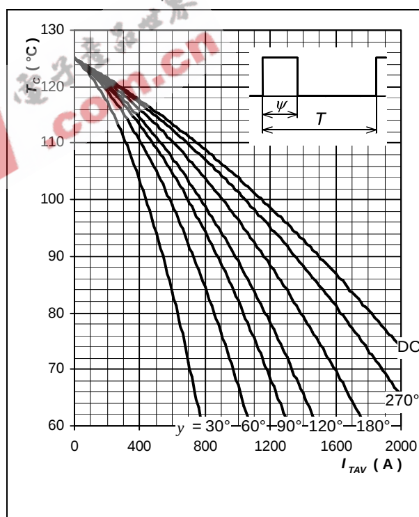
Fig. 9 Max. case temperature vs. average forward current, square waveform, f = 50 \text{ Hz} , T = 1/f
