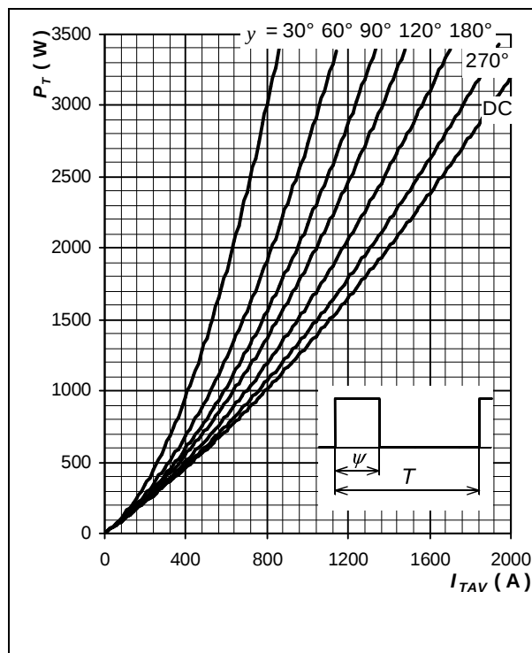
Fig. 7 Forward power loss vs. average forward current, square waveform, f = 50 \text{ Hz} , T = 1/f
