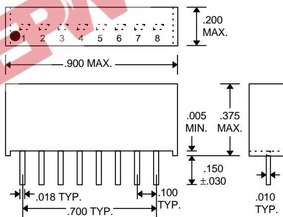
DDU222F-xxM (Military)
