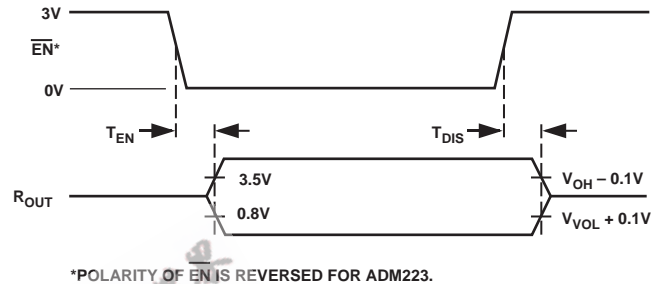
Figure 35. Enable Timing
