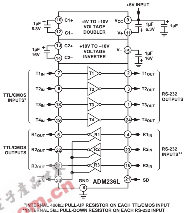
Figure 14. ADM236L Typical Operating Circuit
