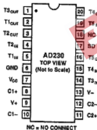
Figure 1. AD230 DIP/SOIC Pin Configuration
