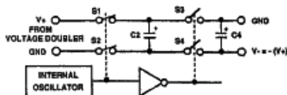
Figure 24. Charge-Pump Voltage Inverter
