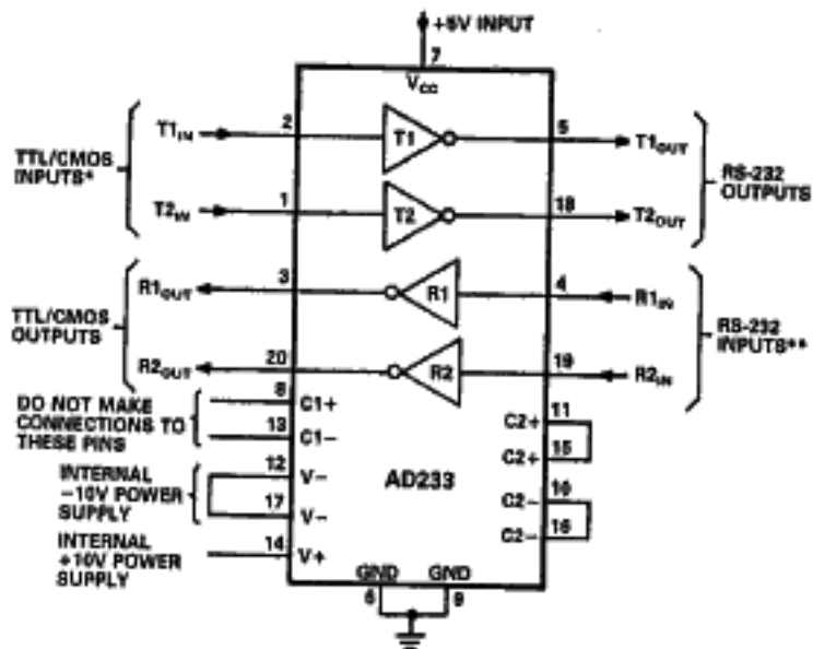
Figure 8. AD233 Typical Operating Circuit
