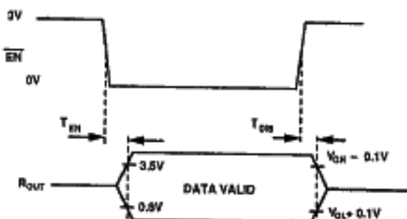
Figure 25. Enable Timing
