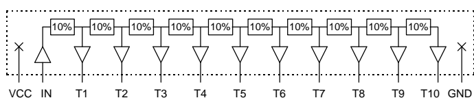
Functional diagram for dash numbers \geq 20
