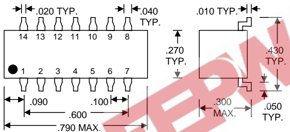
DDU4C-xxA2 (Commercial Gull-Wing)
