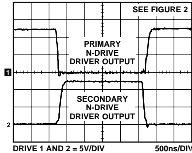
Figure 7. Gate Switching Waveforms
