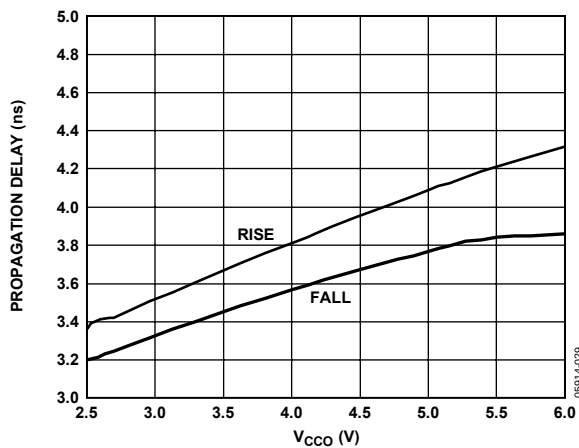
Figure 14. Propagation Delay vs. V_{CCO}
