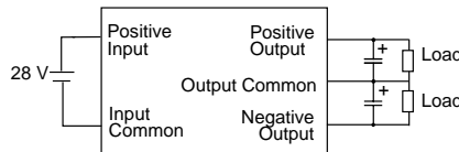
FIGURE 1: DUAL DCH CONVERTER WITH EXTERNAL CAPACITORS
