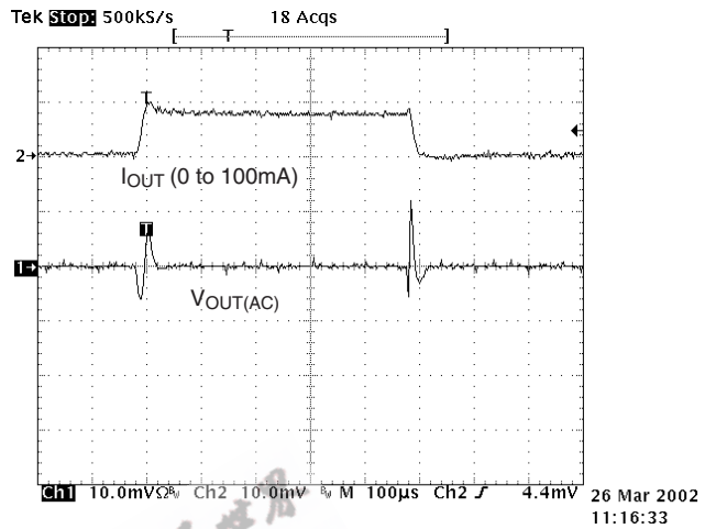
Load Transient Response V_{IN} = V_{OUT} + 1V, CN=0
