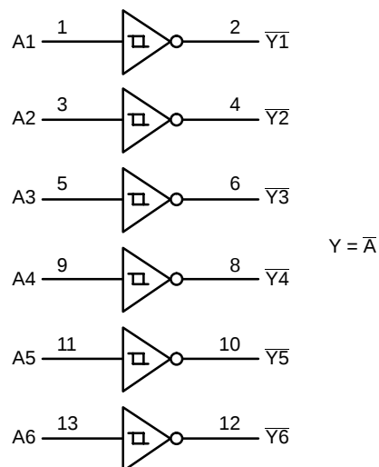
Figure 2. Logic Diagram
