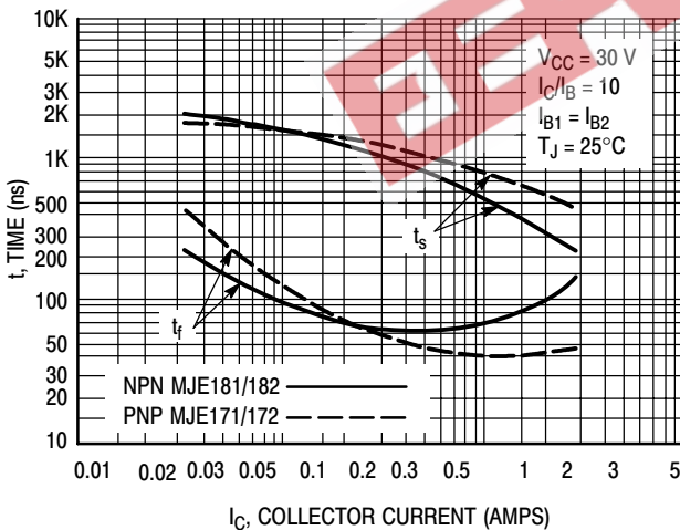
Figure 7. Turn-Off Time
