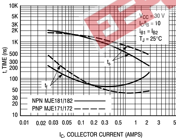
Figure 7. Turn-Off Time
