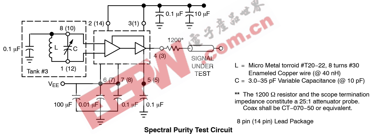
Figure 16. Spectral Purity of Signal Output for 200 MHz Testing
