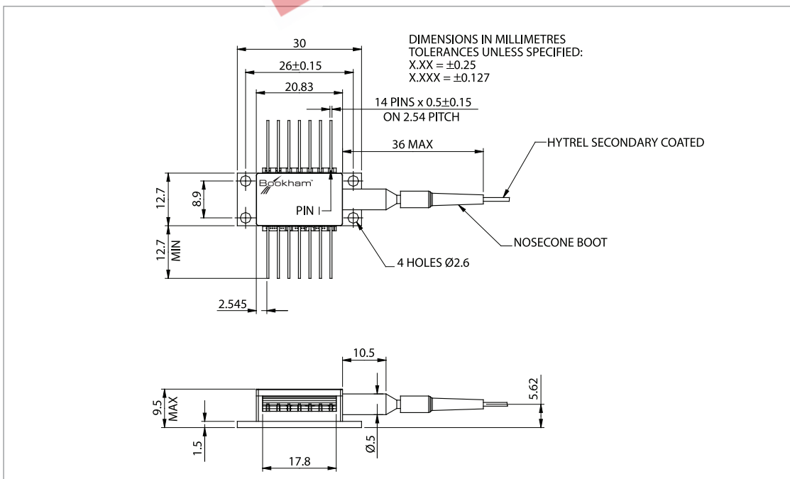
Figure 1: Outline Drawing.
