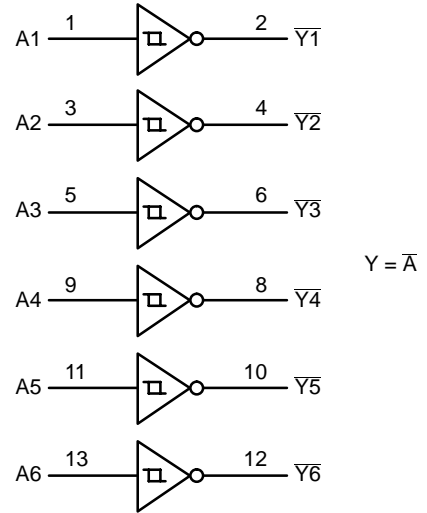
Figure 2. Logic Diagram
