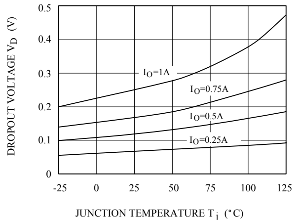
Fig.8 T_j - V_D
