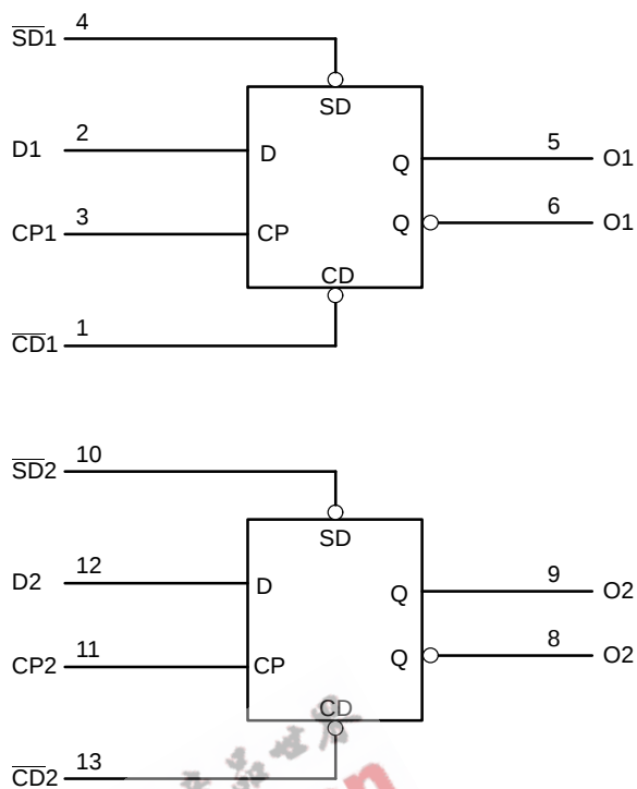
Figure 2. Logic Diagram
