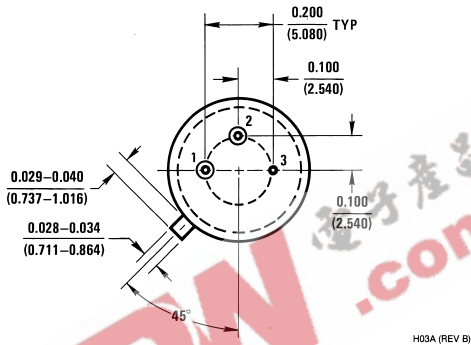
Metal Can Package (H) Order Number LM109H, LM109H/883 or LM309H NS Package Number H03A
