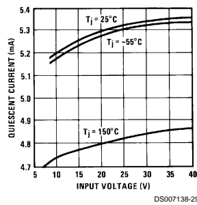
Quiescent Current
