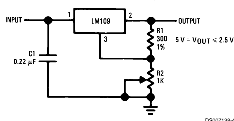
Adjustable Output Regulator
