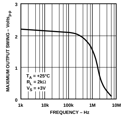
Figure 9. OP183/OP283 Maximum Output Swing vs. Frequency @ +3 V
