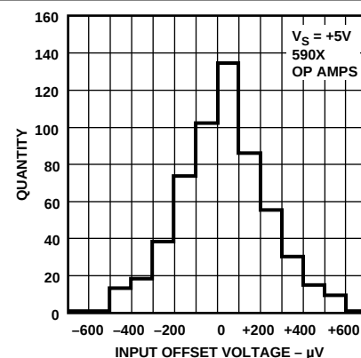
Figure 3. OP283 Input Offset Voltage Distribution @ +5 V
