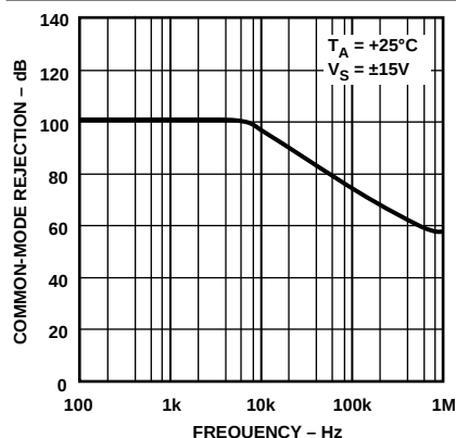
Figure 19. Common-Mode Rejection vs. Frequency
