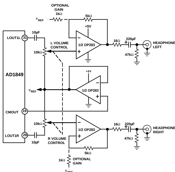
Figure 39. Headphone Output Amplifier for Multimedia Sound Codec
