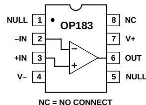
8-Lead Epoxy DIP (P Suffix)
