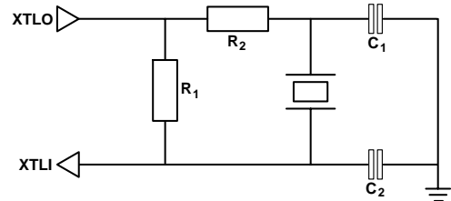
Figure 2: Crystal Oscillator Circuit
