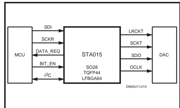
Figure 12. Input from BITSTREAM, Output from I2C
