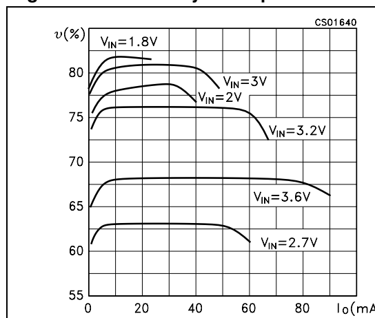
Figure 7. Efficiency vs output current
