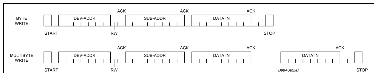
Figure 9. Write Mode Sequence
