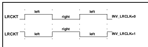
Figure 12. LRCKT Polarity Selection
