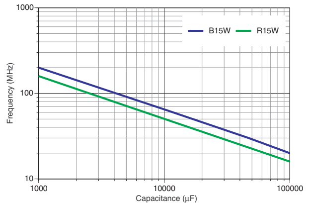
0508 X7R SERIES RESONANT FREQUENCY
