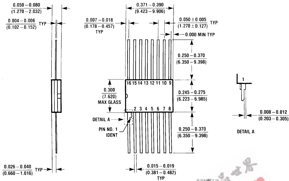
16-Lead Ceramic Flat Package (W) Order Number 54173FMBQ or DM54173W NS Package Number W16A
