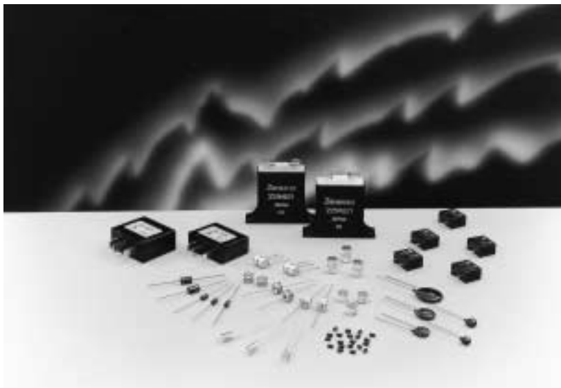
SURGE ABSORBERS
