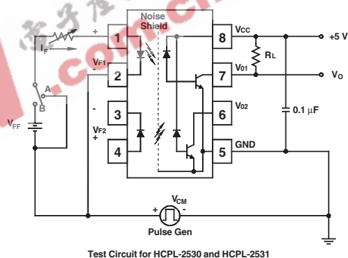
Test Circuit for HCPL-2530 and HCPL-2531
