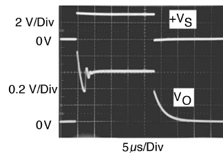
Start-Up Response
