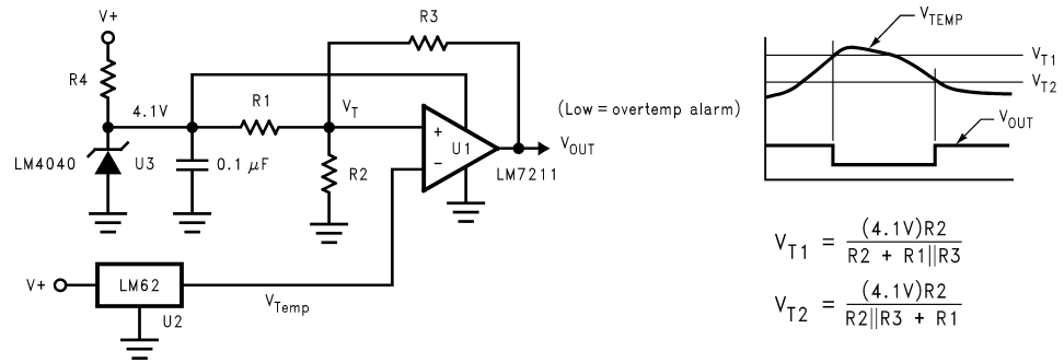
FIGURE 7. Centigrade Thermostat
