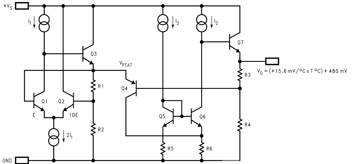
FIGURE 6. Simplified Schematic
