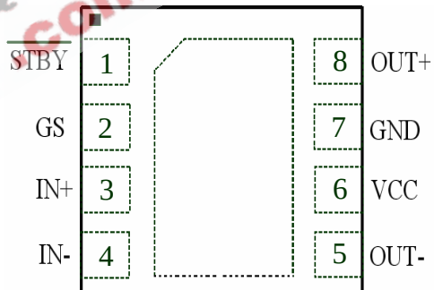
TS2007IQT - DFN8
