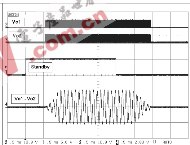
Figure 49. Startup and shutdown phase V_{CC}=5V , G=12dB , C_{in}=1\mu F , V_{in}=1V_{pp} , F=10kHz
