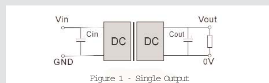
Figure 1 - Single Output
