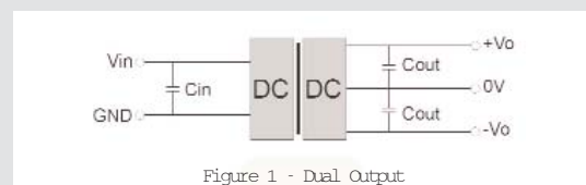
Figure 1 - Dual Output
