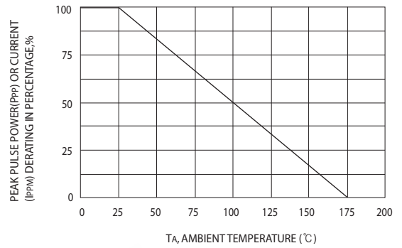
FIG.2-PULSE DERATING CURVE
