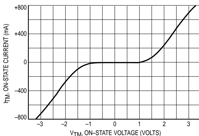
Figure 2. On-State Characteristics
