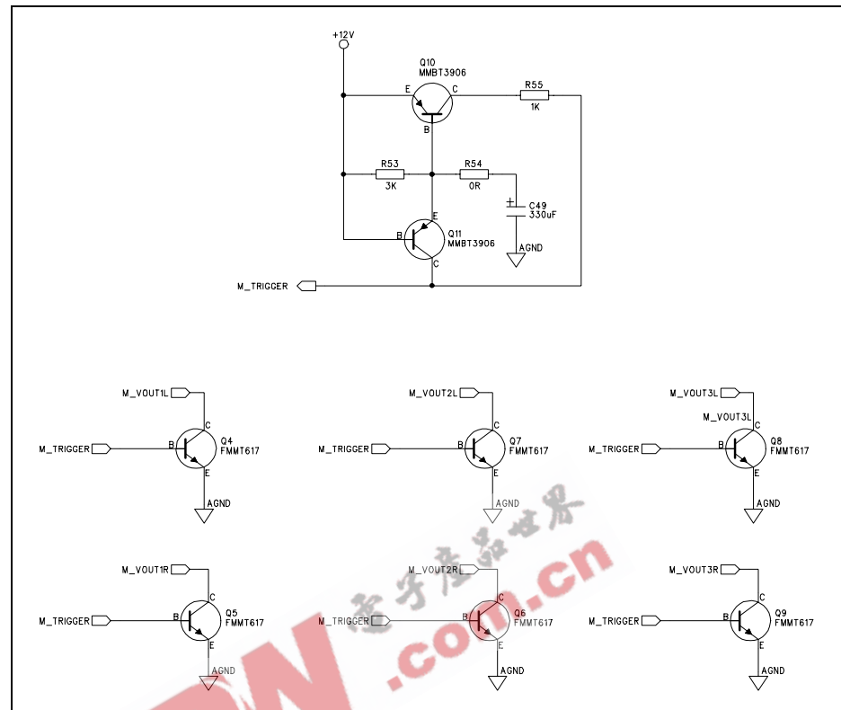
Figure 52 Output Clamp Circuit
